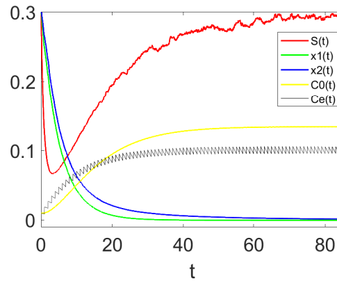
Figure 2. The trajectories of the solution of the stochastic model
