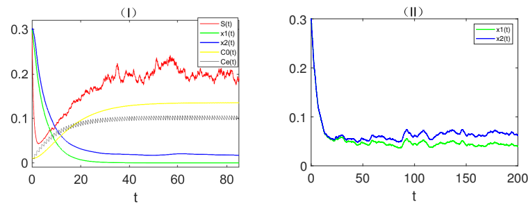
Figure 3. Figure 3(I) is the trajectory of the solution of model (1.1), and Figure 3(II) is the trajectories of x_1(t) and x_2(t) .
