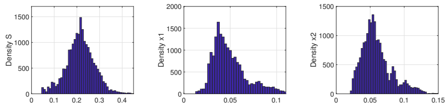
Figure 4. The probability density of S(t) , x_1(t) and x_2(t)
