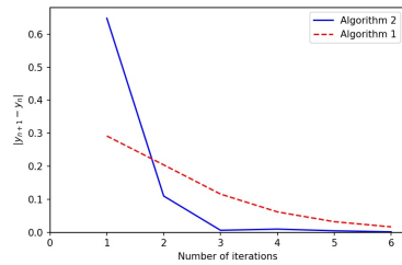
Figure 4(a). Some iterates of Algorithms 1 and 2 choosing y_0(t) = t + 1 and y_1(t) = \sin t
