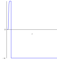
Figure 5. The diagram of function \bar{g}_{36}(r)
