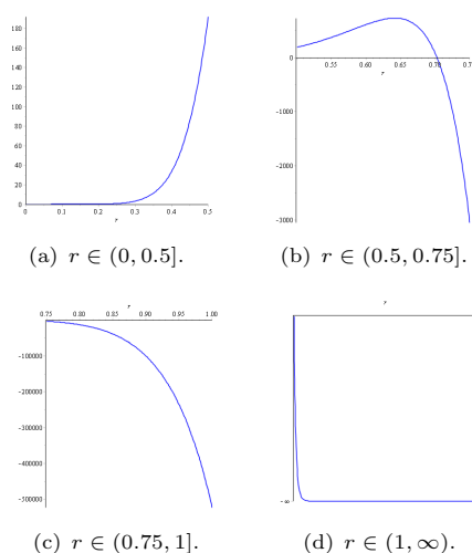
Figure 6. The graphic of function \bar{g}_{35}(r)
